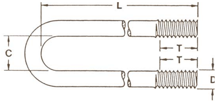
U-Bolt, Round Bend (DxLxCxT)
